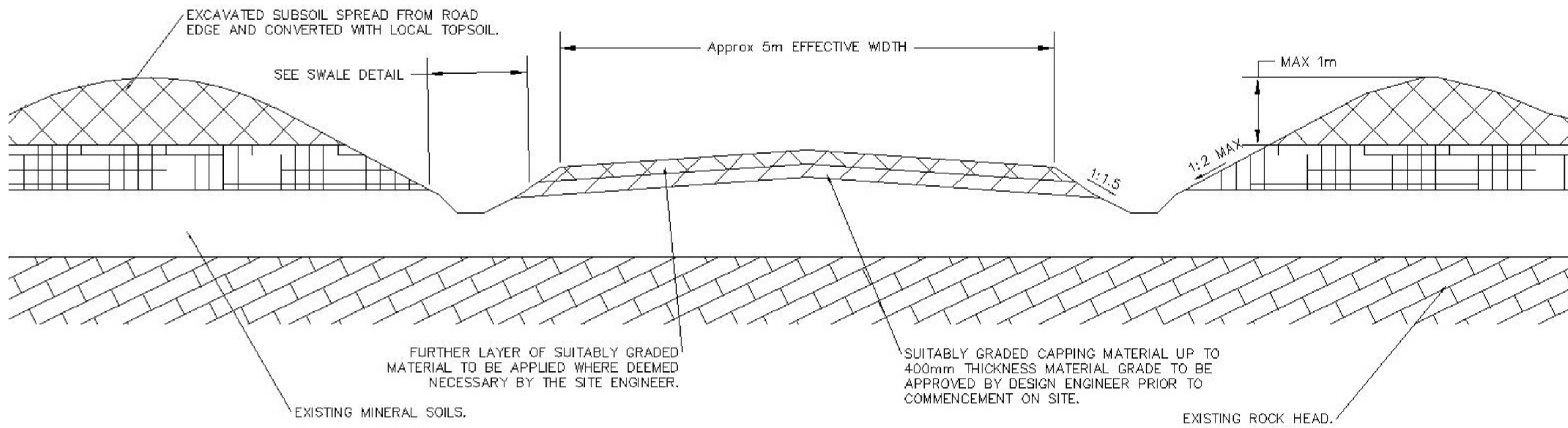
TYPICAL TRACK FORMATION ON OVERBURDEN SOIL
