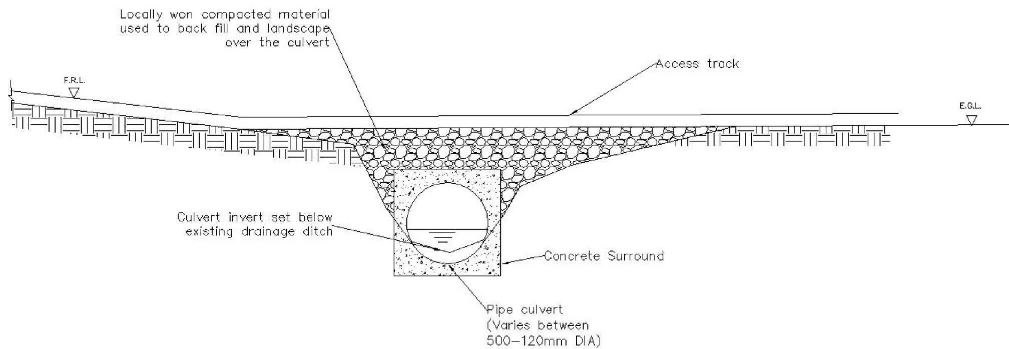
INDICATIVE CLOSED PIPE DRAINAGE DITCH CROSSING
