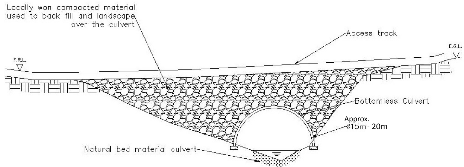
INDICATIVE BOTTOMLESS ARCH WATERCOURSE CROSSING
